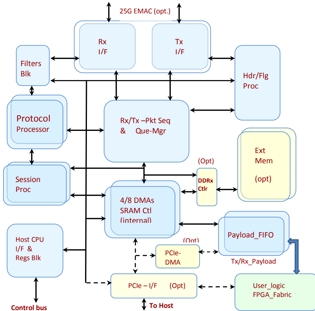
25G TCP Offload Engine (Simplified Block Diagram)
