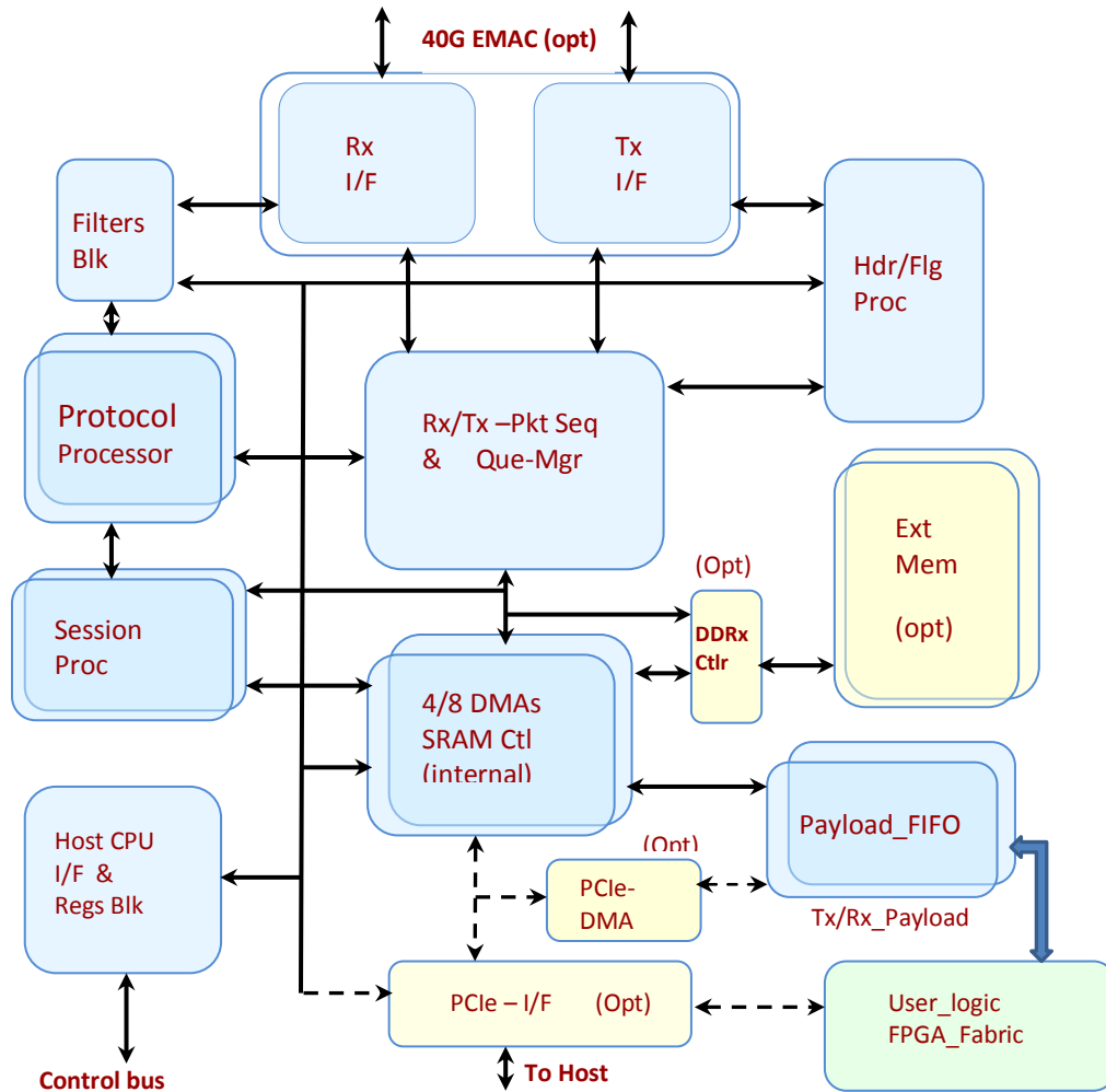
40G TCP Offload Engine + EMAC (Simplified Block Diagram)
